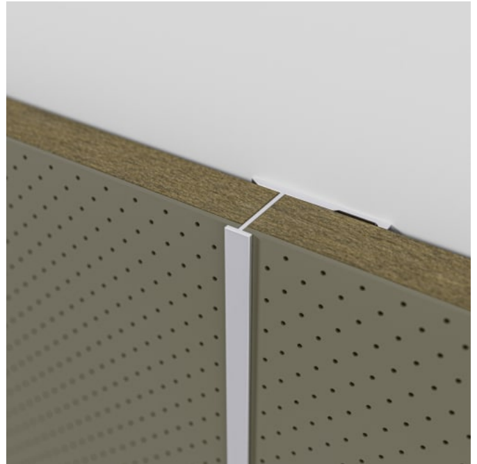
Joiner Trim Install Detail
